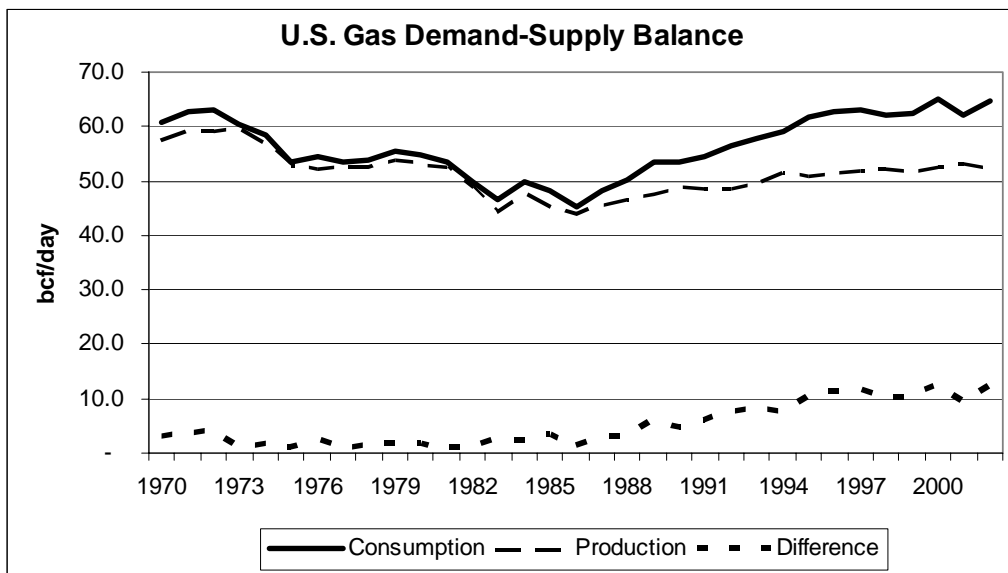
Figure 3. U.S. Gas Demand-Supply Balance
